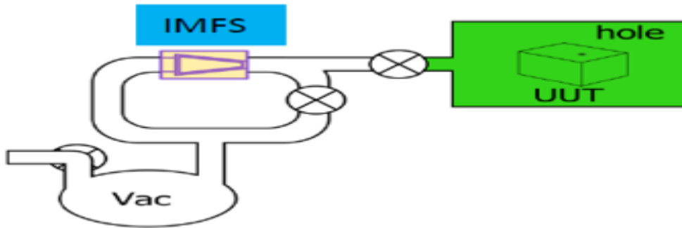
1 Standby - Vacuum Reservoir: P_0 - IGLS: no flow
